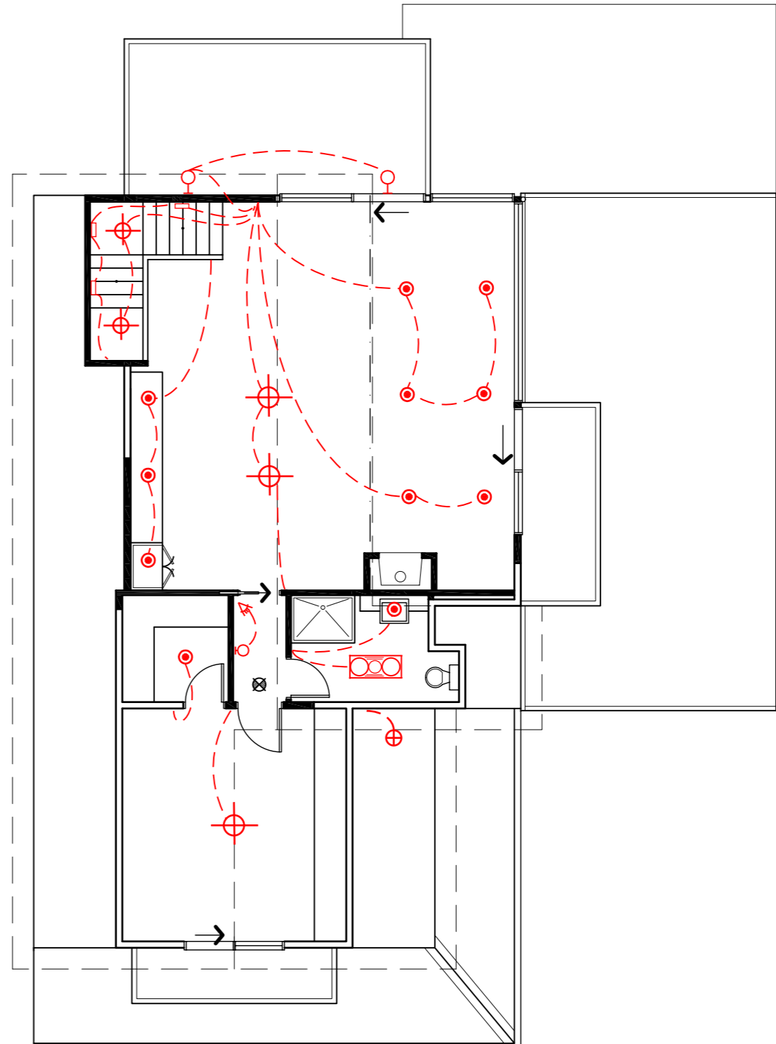
upper floor electrical plan scale 1:100
