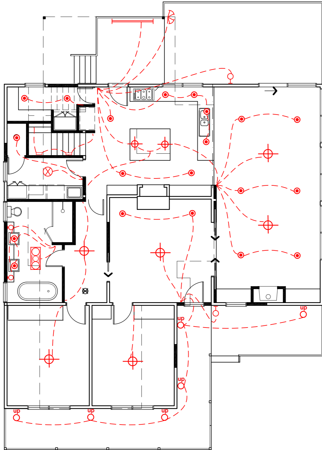
ground floor electrical plan scale 1:100
